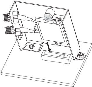
5 Insert WiFi card to M.2 (E Key) socket and cover the outer casing.
