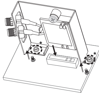
6 Fixing screw. ★ Screws type The bottom of the Mainboard locks the iron piece.
