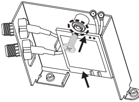
3 Place the wifi cables on the sponge pad, insert the wifi card and tighten the screws.
