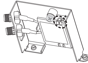
4 WiFi cables connection WiFi card. ★ A screwdriver can be used to assist snap in fastening the connector.
